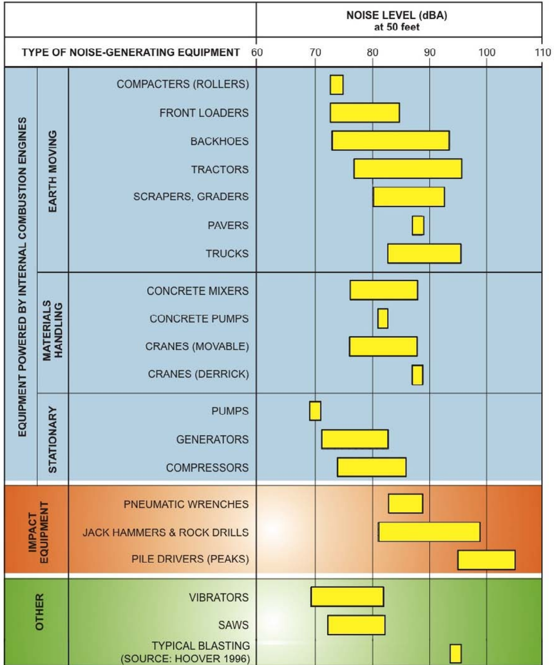
Figure 3.4-1: Construction Equipment Noise Levels
